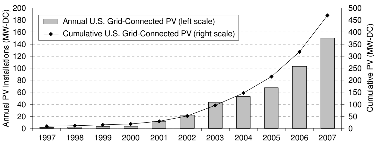
Figure 1. Annual and Cumulative Grid-Connected PV Capacity in the U.S.
